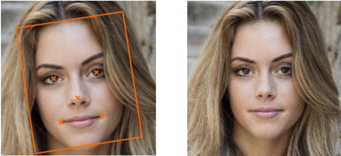
Figure 2: Face warping
