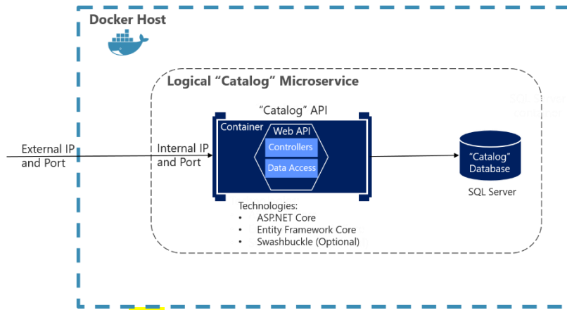
Figure X-XX. Simple data-driven/CRUD microservice design diagram
