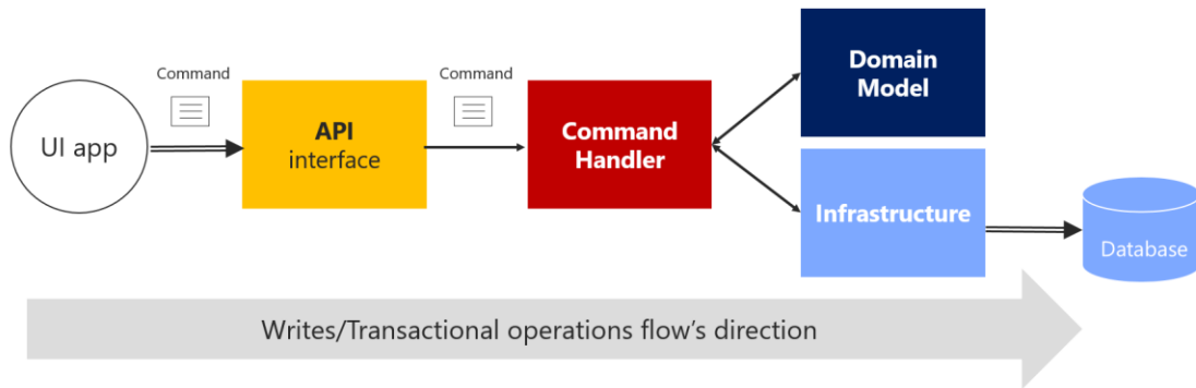
Figure 9-20. High-level view of the commands or “transactional side” in a CQRS pattern
