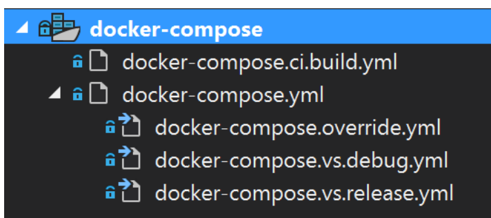
Figure 8-11. docker-compose files in Visual Studio 2017
