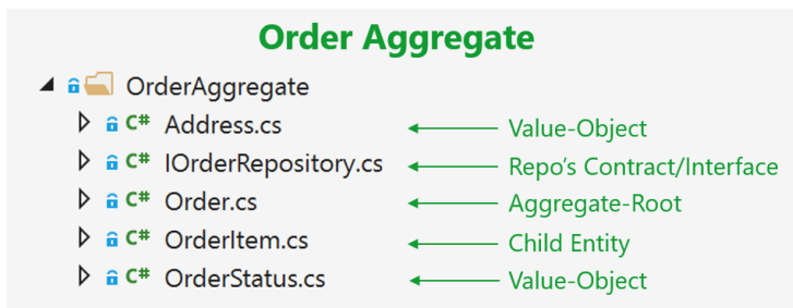
Figure 9-11. The order aggregate in Visual Studio solution
