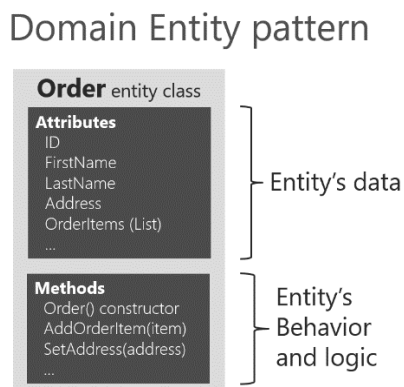
Figure 9-8. Example of a domain entity design implementing data plus behavior
