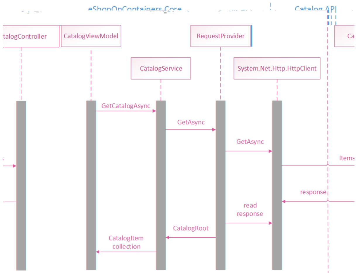
Figure 10-1: Retrieving data from the catalog microservice
