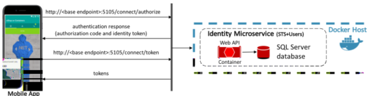
Figure 9-2: High-level overview of the sign-in process
