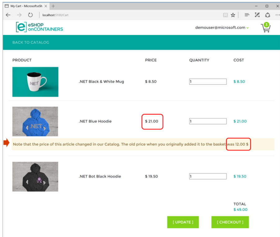
Figure X-XX. Detecting item price change in basket communicated by integration events
