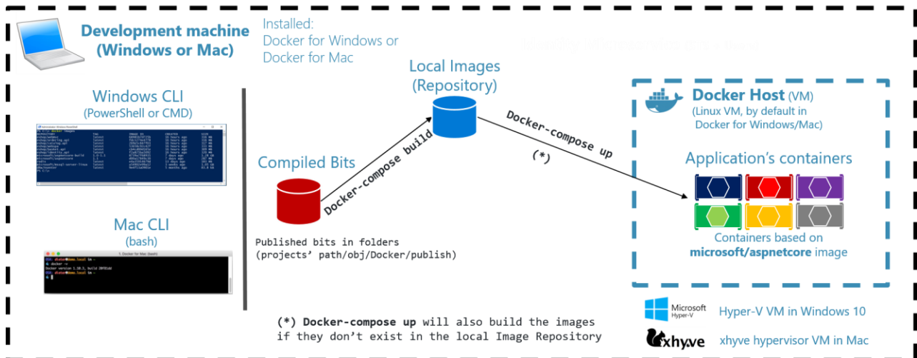
Figure X-XX. Building Docker images and running the containers
