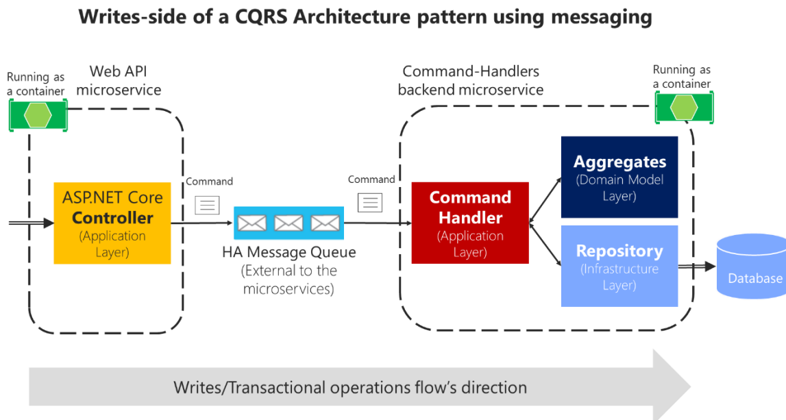
Figure X-XX. Using Message Queues with CQRS Commands
