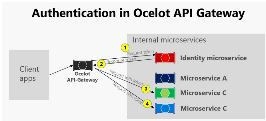
Figure 6-39. Authentication in Ocelot
