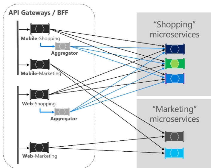
Figure 6-37. Zoom in vision of the Aggregator services
