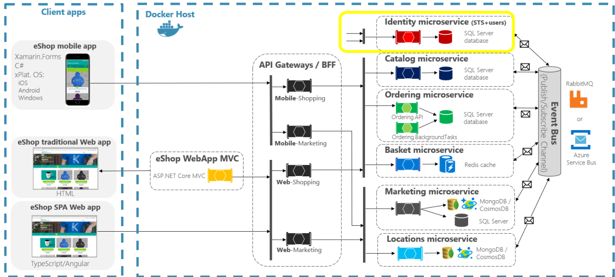
Figure 6-38. Position of the Identity service in eShopOnContainers
