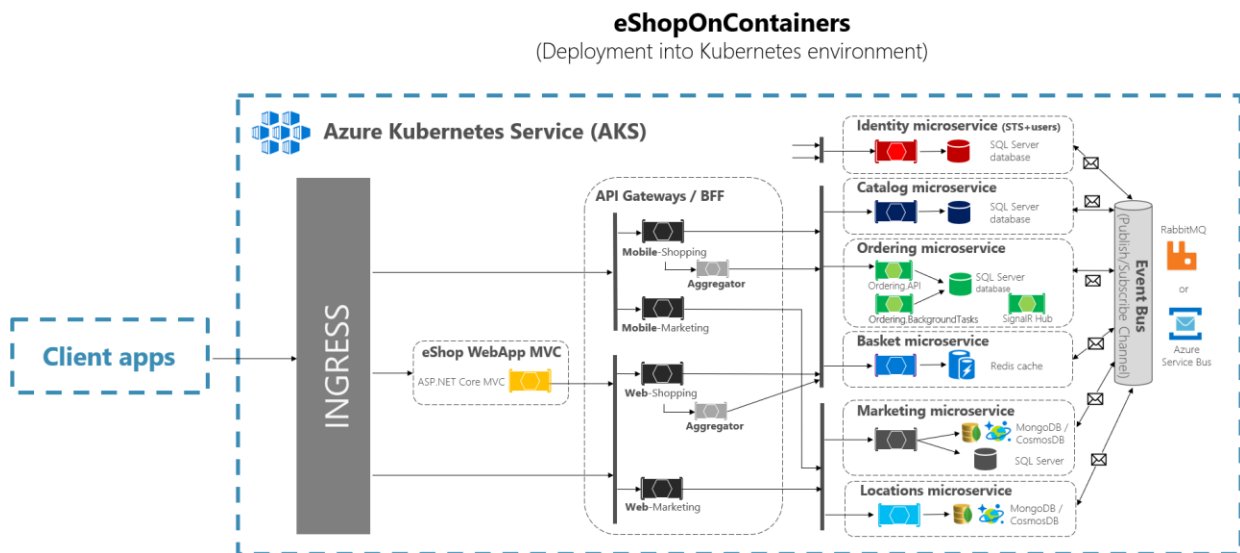
Figure 6-40. The ingress tier in eShopOnContainers when deployed into Kubernetes
