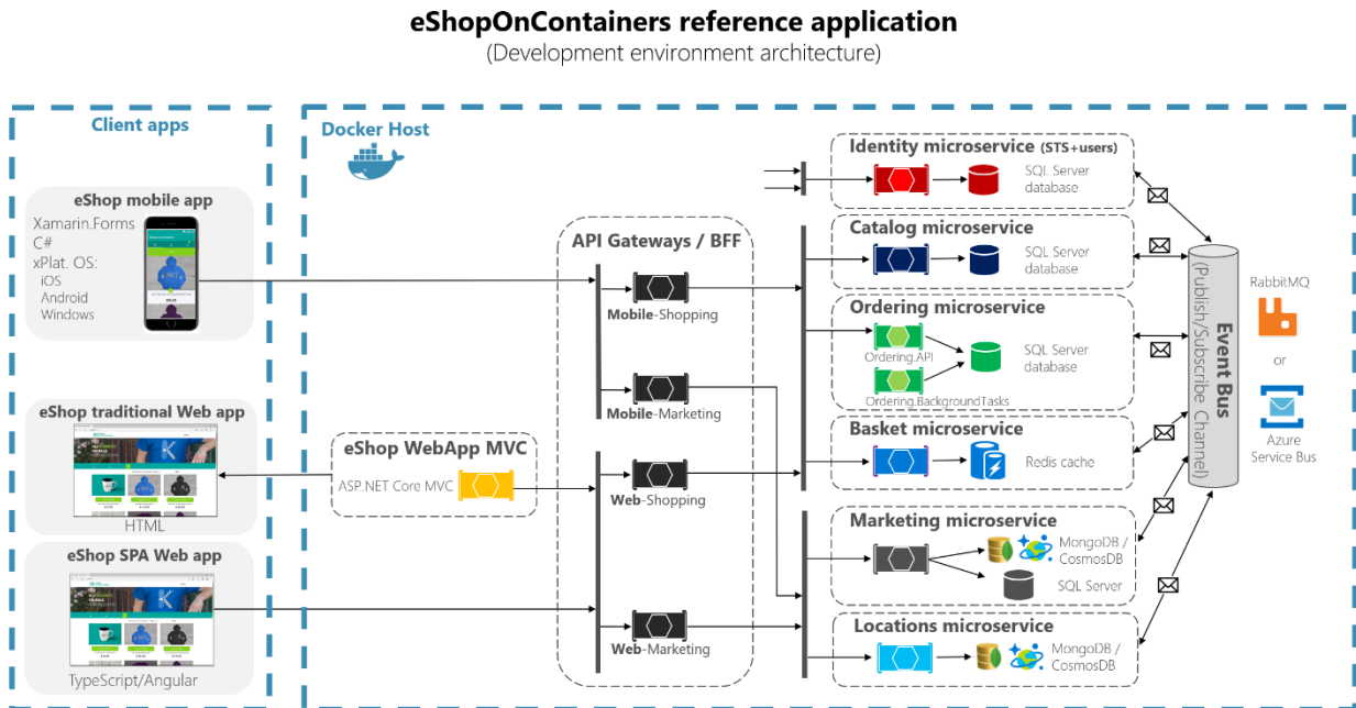
Figure 6-27. eShopOnContainers architecture with API Gateways
