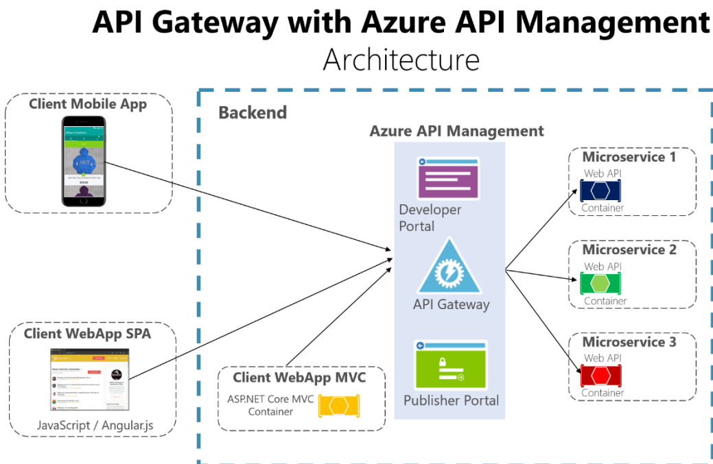
Figure 4-14. Using Azure API Management for your API Gateway
