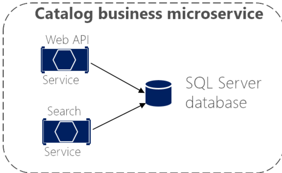
Figure 4-8. Business microservice with several physical services
