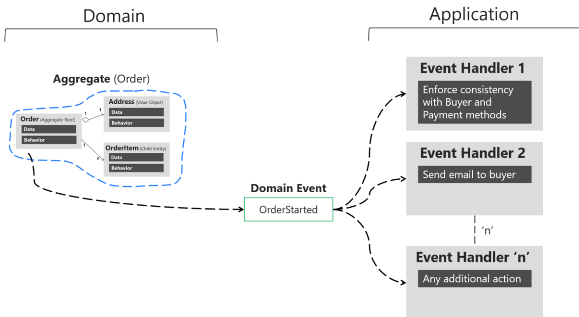
Figure X-XX. Handling multiple actions per domain event
