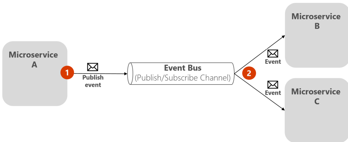
Figure X-XX. Publish/Subscribe basics with an Event Bus
