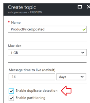
Figure X-XX. Duplication Detection in Azure SB
