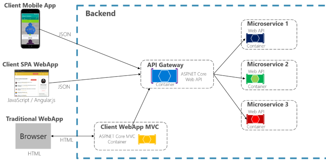
Figure 4-13. Using an API Gateway implemented as a custom Web API service
