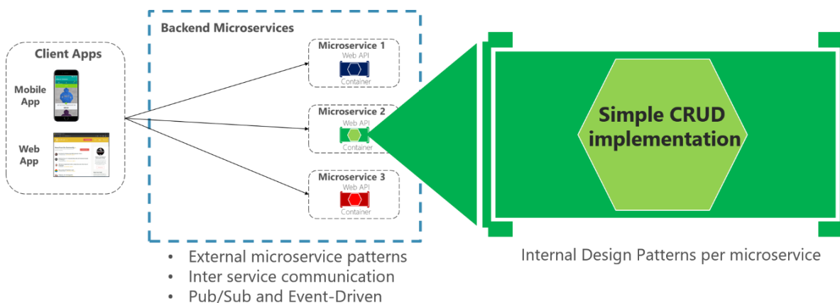
Figure 6-4. Internal design for simple CRUD microservices
