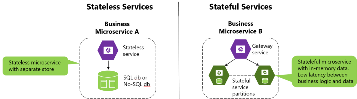
Figure 4-30. Stateless versus stateful microservices
