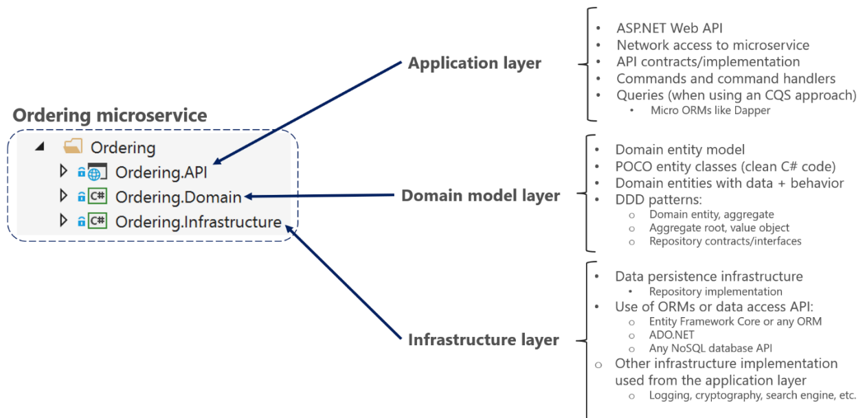
Figure 7-5. DDD layers in the ordering microservice in eShopOnContainers
