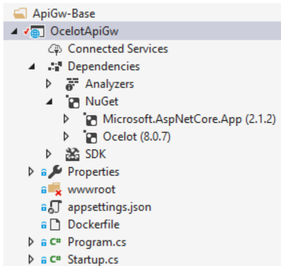
Figure 6-32. The OcelotApiGw base project in eShopOnContainers
