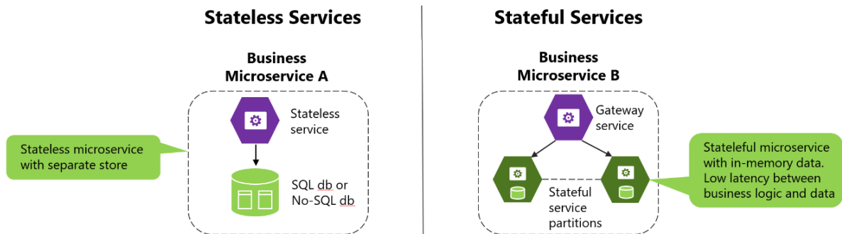
Figure 4-31. Stateless versus stateful microservices
