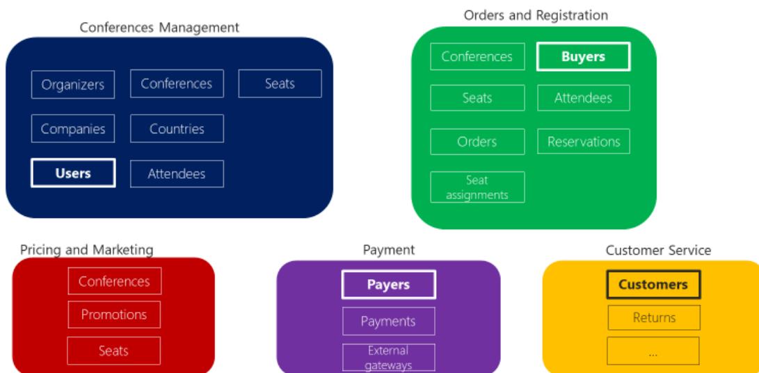
Figure 4-10. Identifying entities and microservice model boundaries
