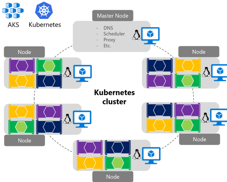
Figure 4-24. Kubernetes cluster's simplified structure and topology
