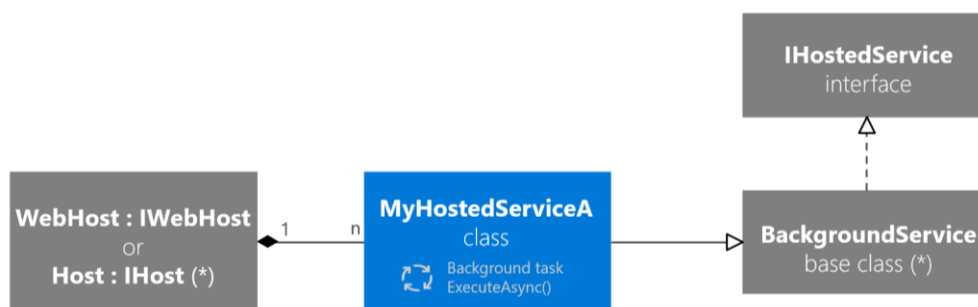
Figure 6-27. Class diagram showing the multiple classes and interfaces related to IHostedService
