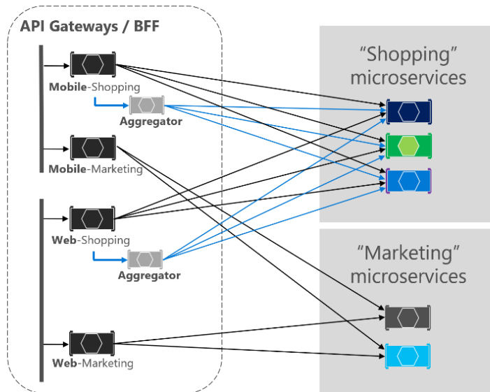
Figure 6-38. Zoom in vision of the Aggregator services
