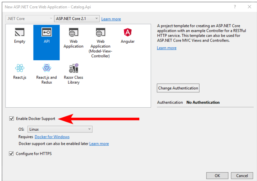
Figure 5-3. Enabling Docker Support when creating a new project in Visual Studio 2017
