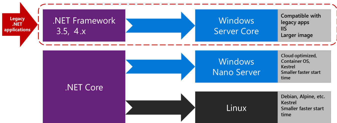
Figure 3-1. Operating systems to target depending on versions of the .NET framework
