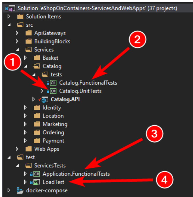
Figure 6-25. Test folder structure in eShopOnContainers
