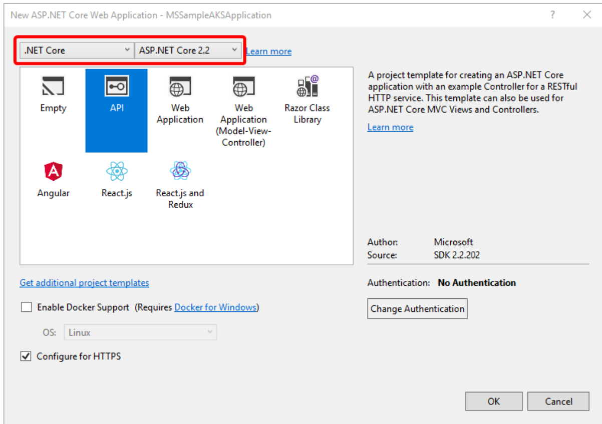
Figure 4-37. Selecting ASP.NET CORE 2.2 and Web API project type
