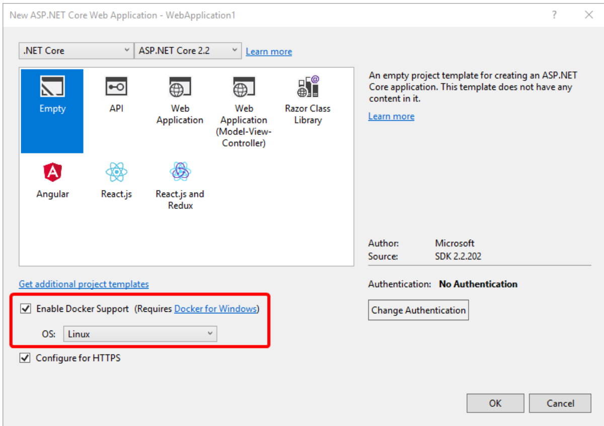
Figure 4-32. Enable Docker support during project creation in Visual Studio 2017
