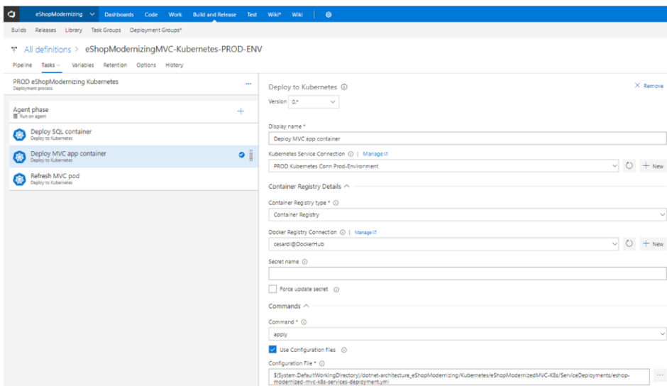
Figure 5-14. Release/CD pipeline in Azure DevOps Services deploying to a Kubernetes cluster
