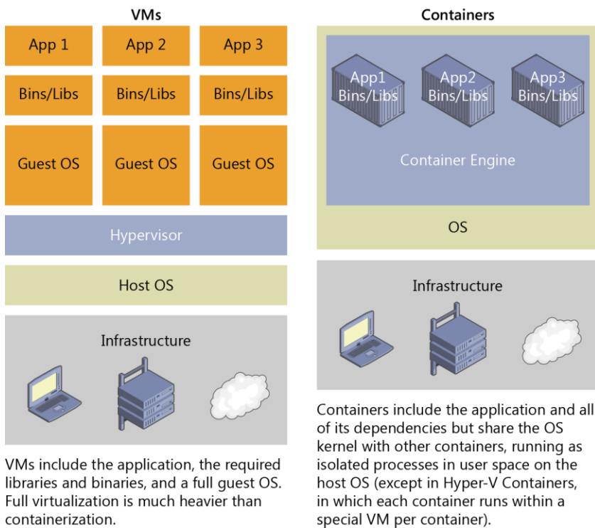
Figure 1-3. Comparison of traditional virtual machines to Docker containers
