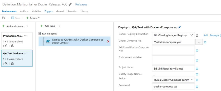
Figure 5-8. Configuring Azure DevOps Services Docker Compose tasks from Azure DevOps Services Release Management
