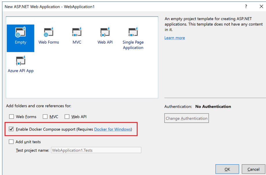
Figure 4-33. Enabling Docker Compose support for an ASP.NET project in Visual Studio 2017
