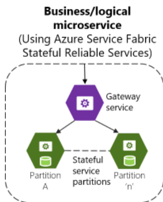
Figure 4-11. Business microservice with several stateful service instances and a custom gateway front end
