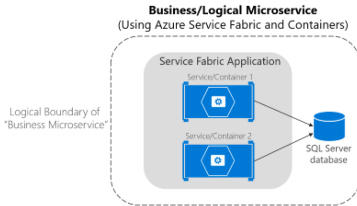
Figure 4-12. Business microservice with several services (containers) in Service Fabric
