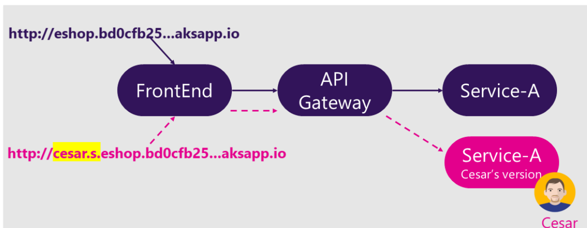
Figure 4-9. Using multiple spaces in Azure Dev Spaces
