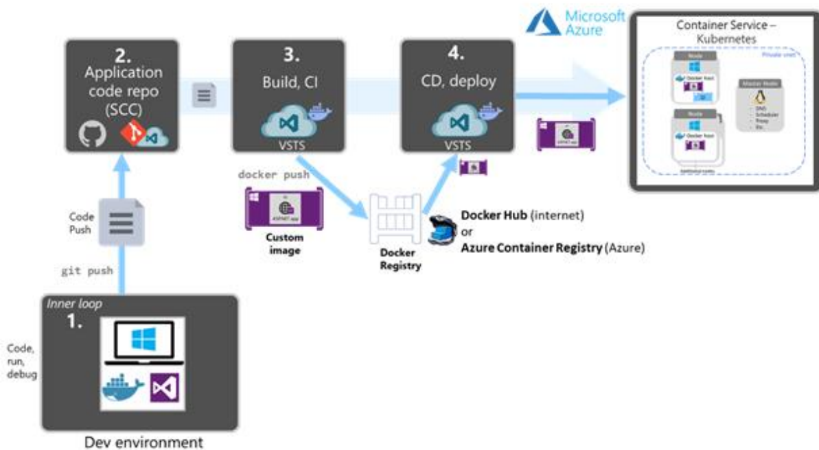
Figure 5-12. CI/CD scenario creating Docker images and deploying to a Kubernetes cluster in Azure
