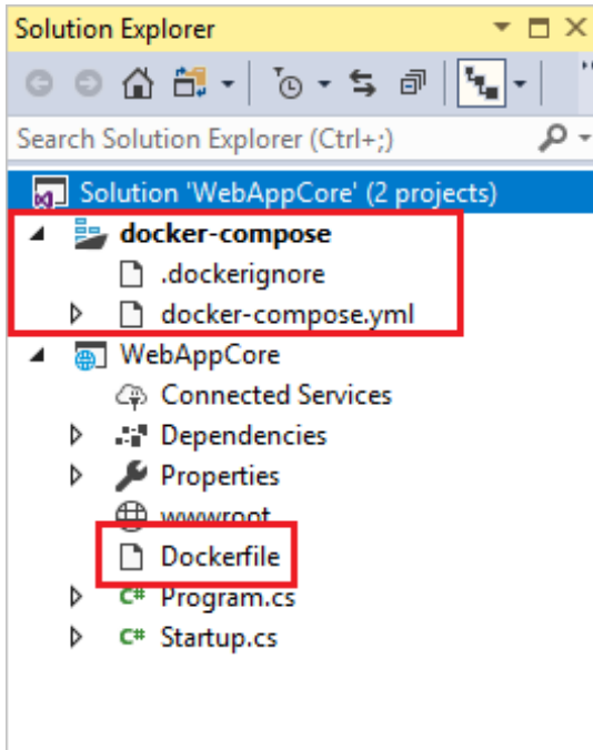
Figure 4-34. Docker files in Solution Explorer in Visual Studio 2017
