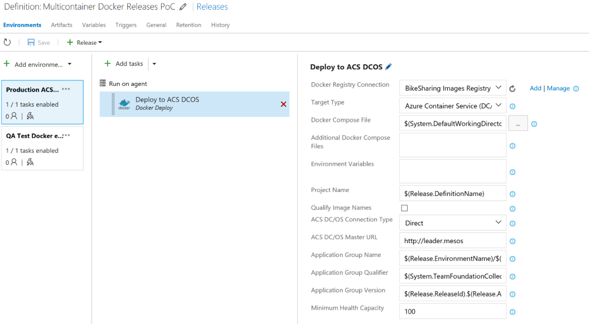
Figure 5-11. Docker Deploy task definition deploying to Azure Container Service DC/OS
