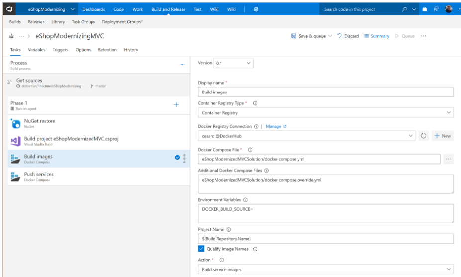
Figure 5-13. Build/CI pipeline in Azure DevOps building Docker images and pushing images to a Docker registry
