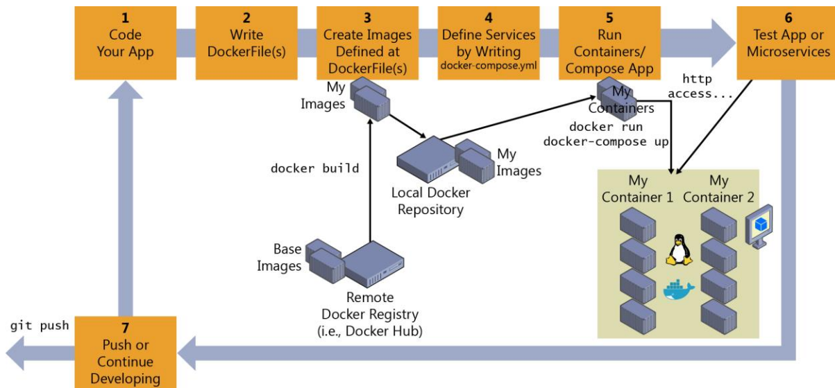
Figure 4-22. High-level workflow for the life cycle for Docker containerized applications using Docker CLI
