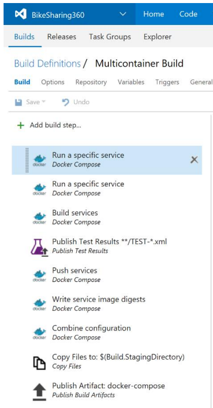
Figure 5-3. The Docker CI pipeline in Azure DevOps Services including Build & Release Templates and associated tasks.
