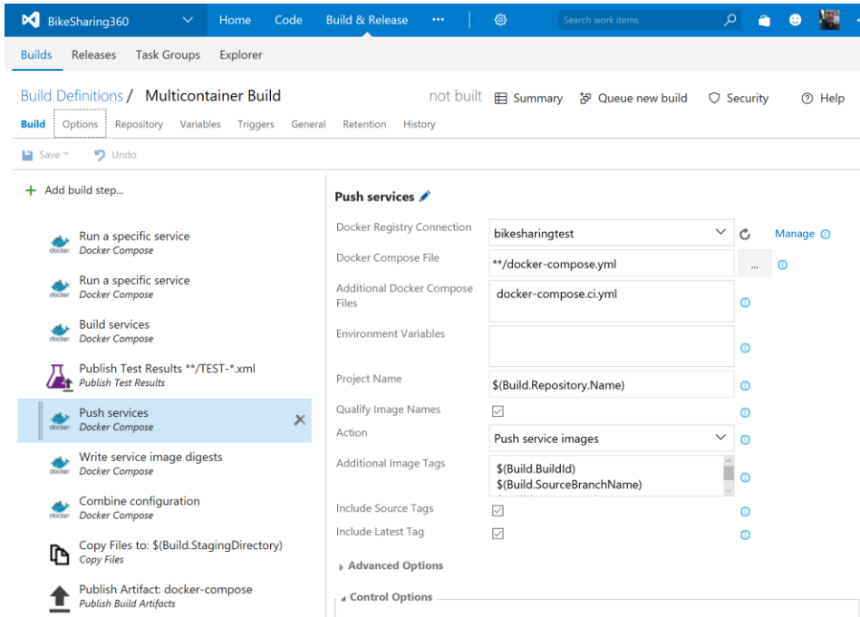
Figure 5-5. Using Azure DevOps Services to publishing custom images to a Docker Registry
