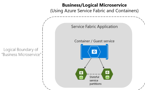
Figure 4-13. Business microservice mapped to a Service Fabric application with containers and stateful services
