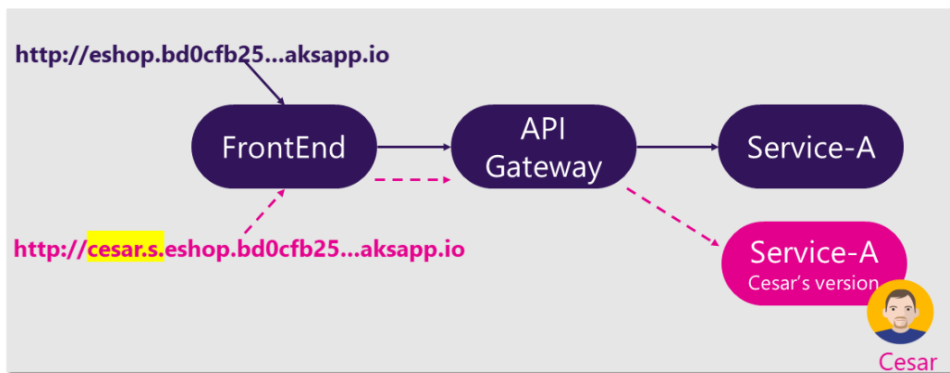
Figure 4-26. Using multiple spaces in Azure Dev Spaces
