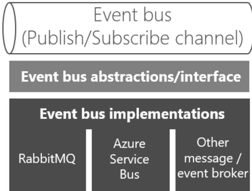
Figure 6- 20. Multiple implementations of an event bus
