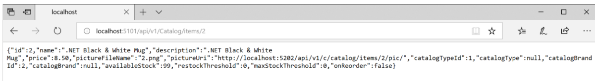
Figure 6-36. Direct access to a microservice for testing purposes
