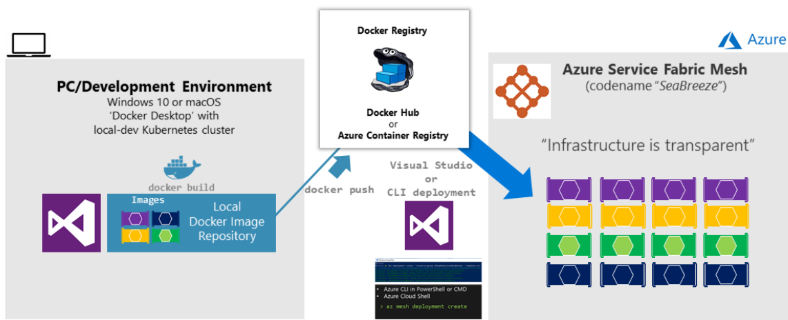
Figure 4-32. Deploying a microservice/containers application to Service Fabric Mesh
