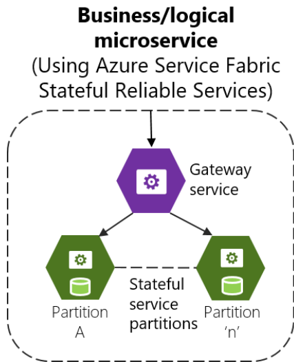
Figure 4-28. Business microservice with several stateful service instances and a custom gateway front-end
