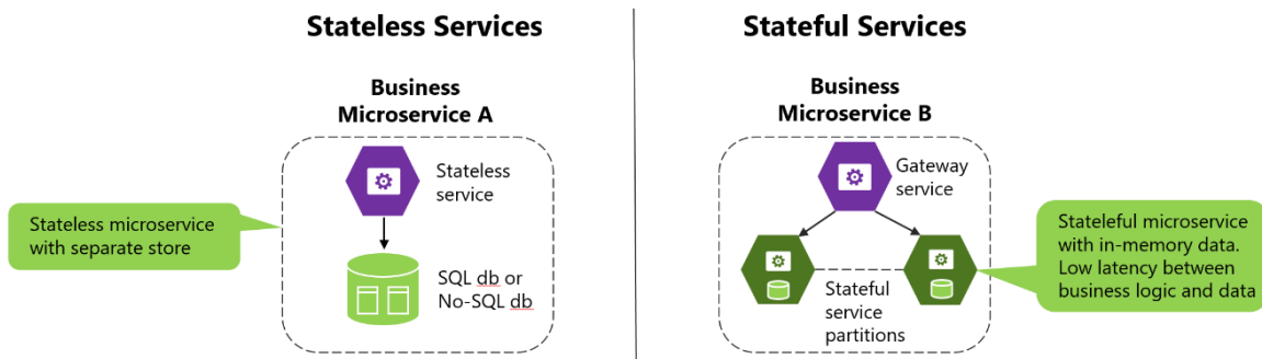
Figure 4-31. Stateless versus stateful microservices
