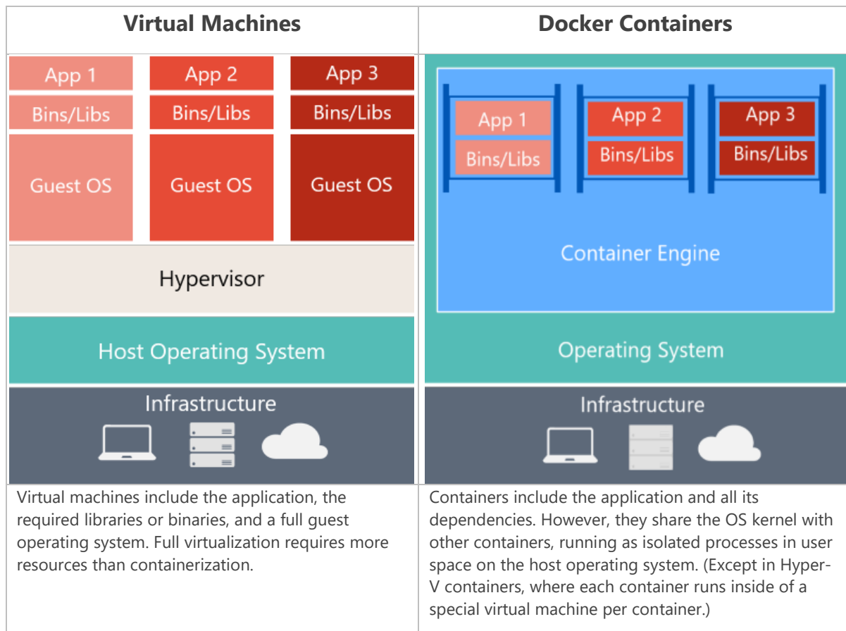
Figure 2-3. Comparison of traditional virtual machines to Docker containers
