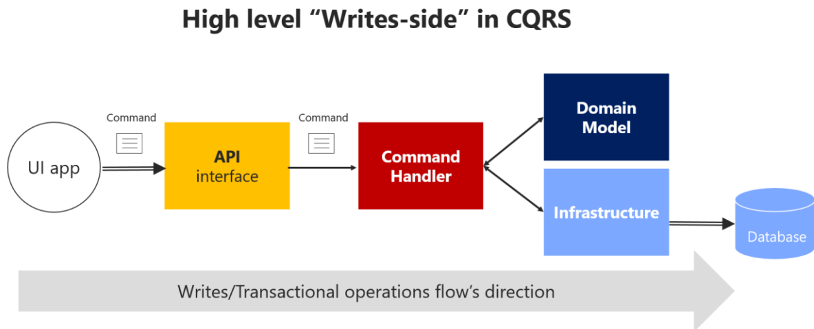
Figure 9-24. High-level view of the commands or “transactional side” in a CQRS pattern
