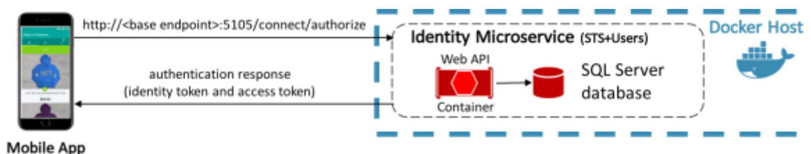
Figure 9-2: High-level overview of the sign-in process
