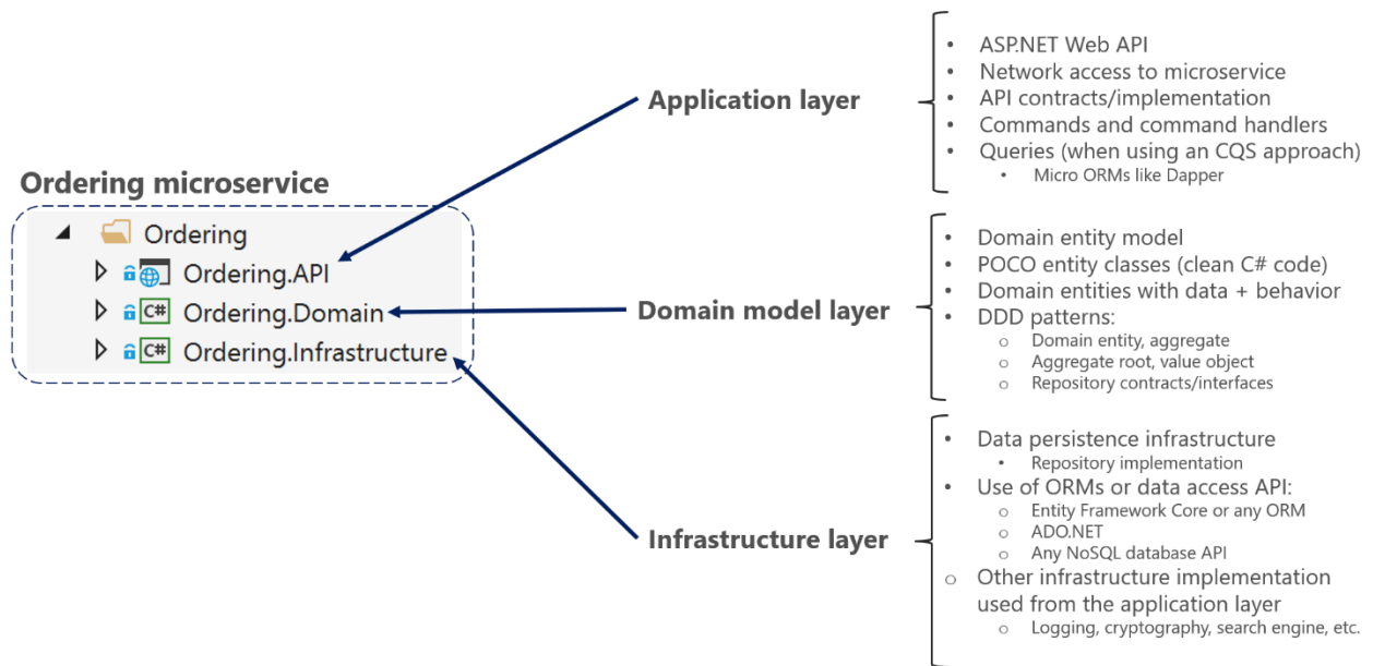
Figure 9-5. DDD layers in the ordering microservice in eShopOnContainers
