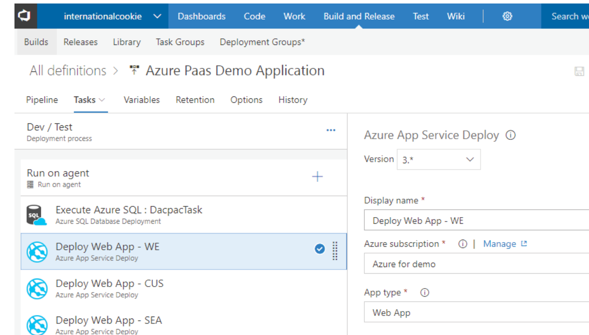
Figure 8: VSTS Release Pipeline
