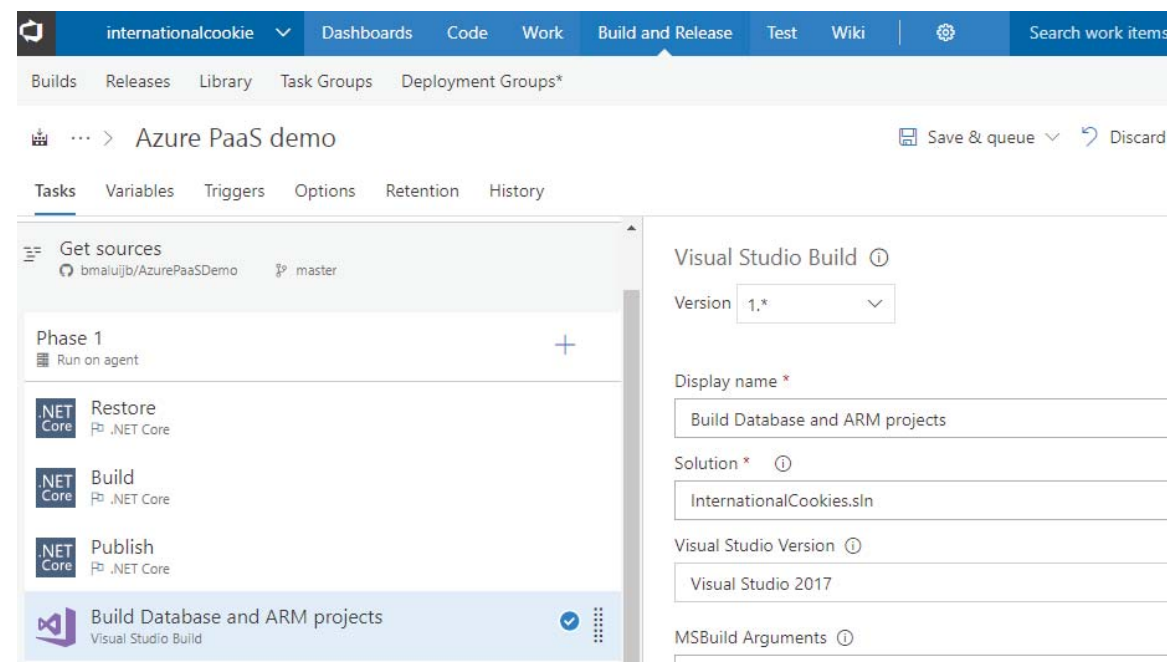
Figure 7: VSTS Build Pipeline
