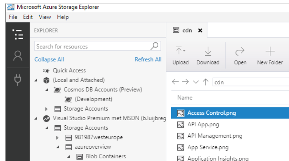
Figure 4: Storage Explorer
